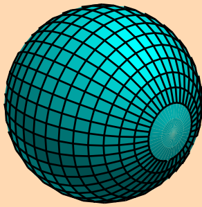
Spherical ground state
