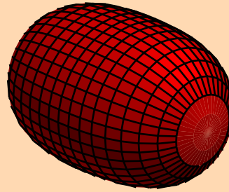
Prolate-triaxial minimum
