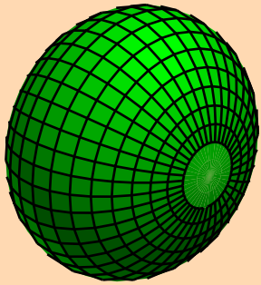
Oblate minimum
