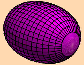
Triaxial saddle
