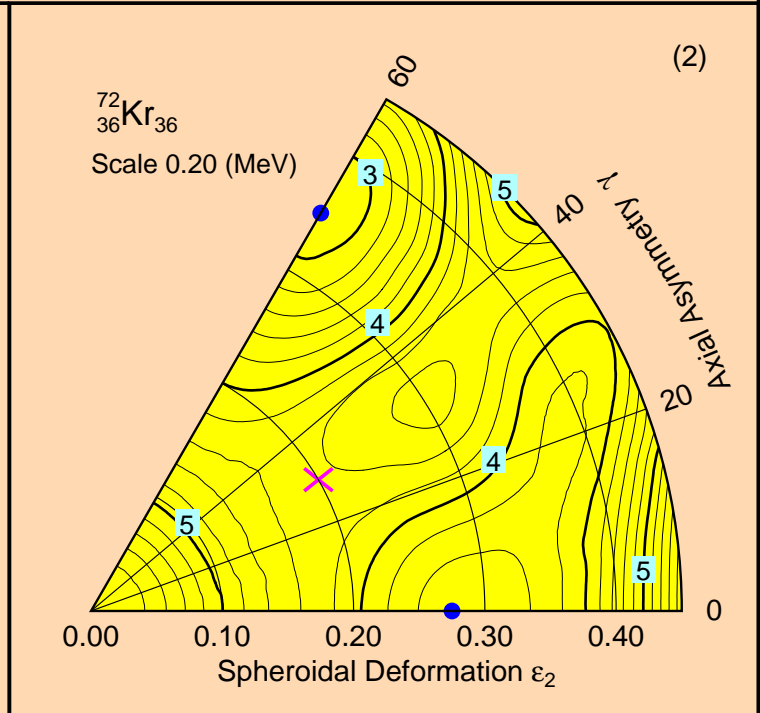
Prolate-triaxial minimum
