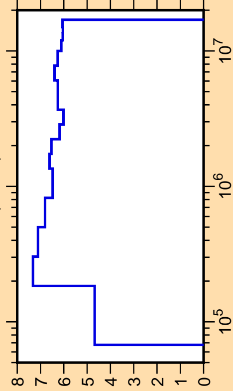
\Delta\sigma/\sigma vs. E for ^{94}\text{Zr}(n,\text{tot.})
