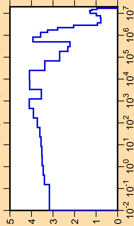
\Delta\sigma/\sigma vs. E for ^{89}\text{Y}(n,\text{tot.})
