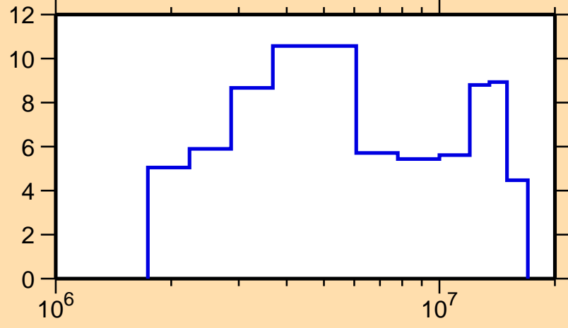
\Delta\sigma/\sigma vs. E for ^{89}\text{Y}(n,el.)
