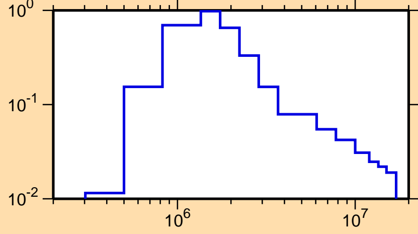
\sigma vs. E for ^{184}\text{W}(\text{mt853})
