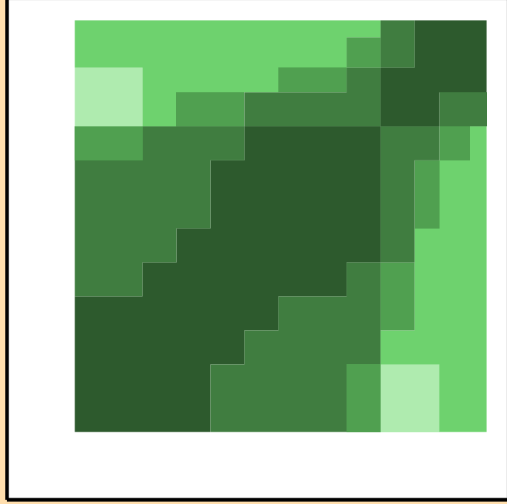
\sigma vs. E for ^{184}\text{W}(\text{mt854})
