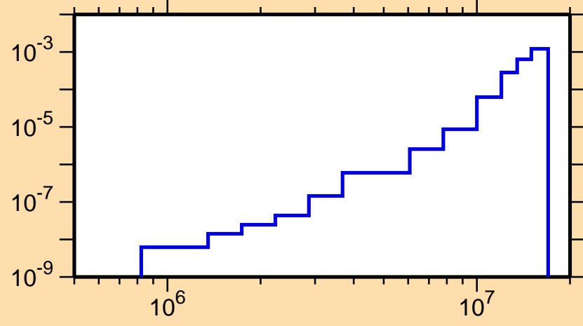
\sigma vs. E for ^{184}\text{W}(\text{mt856})
