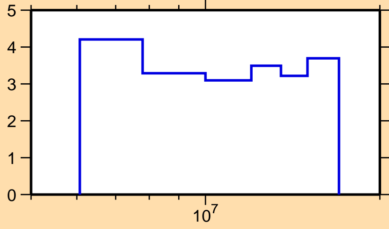
\Delta\sigma/\sigma vs. E for ^{184}\text{W}(\text{mt852})
