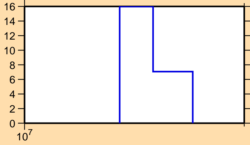
\Delta\sigma/\sigma vs. E for ^{184}\text{W}(n,3n)
