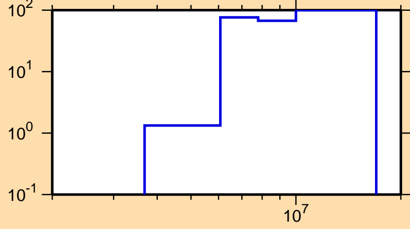
\Delta\sigma/\sigma vs. E for ^{184}\text{W}(\text{mt851})
