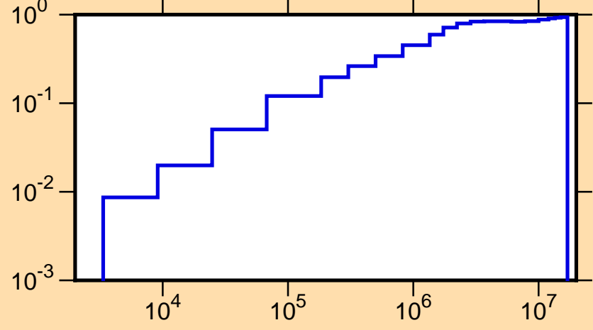
\mu vs. E for ^{182}\text{W}(\text{mt251})
