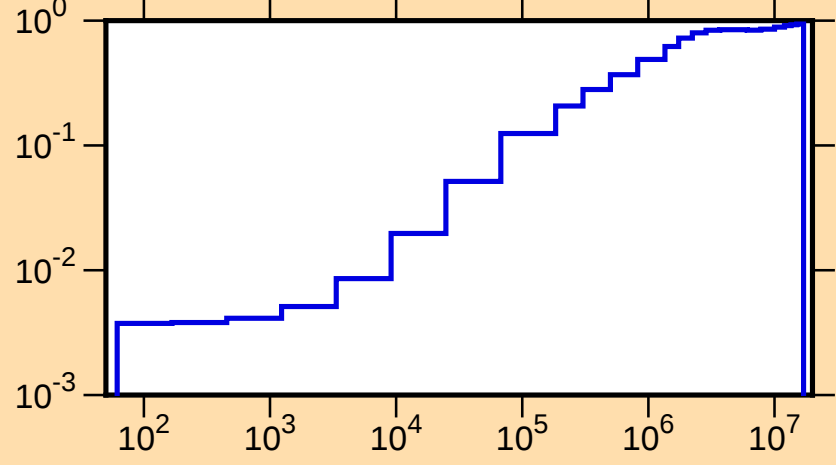
\mu vs. E for ^{180}\text{W}(\text{mt251})
