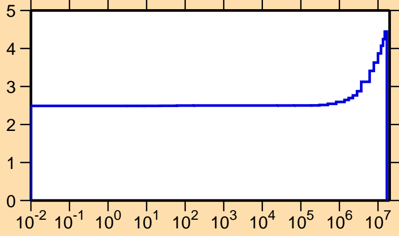
\nu vs. E for ^{233}\text{U} (prompt \nu )
