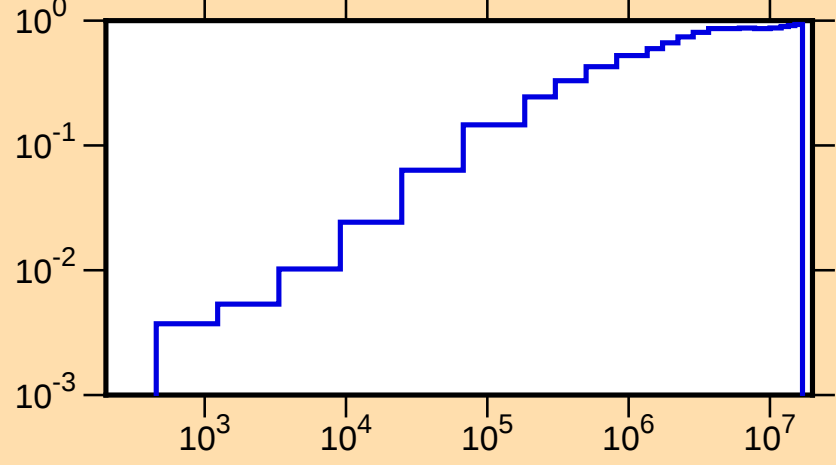
\mu vs. E for ^{232}\text{U}(\text{mt251})
