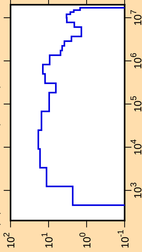
\Delta\mu/\mu vs. E for ^{232}\text{U}(\text{mt251})
