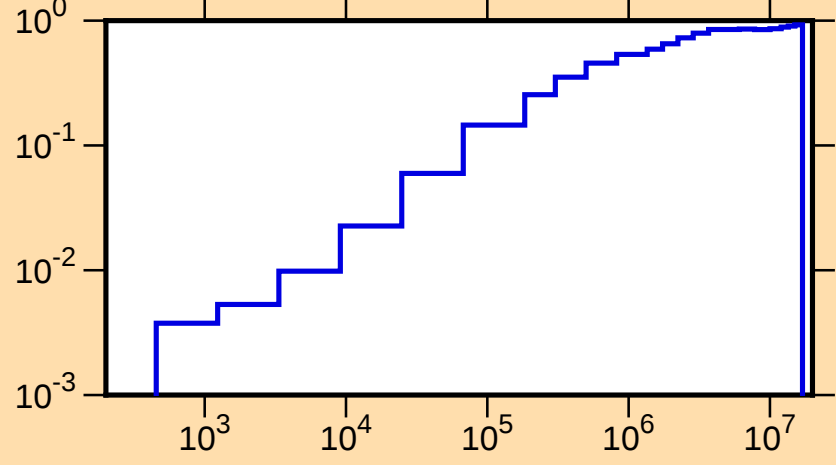
\mu vs. E for ^{231}\text{U}(\text{mt251})
