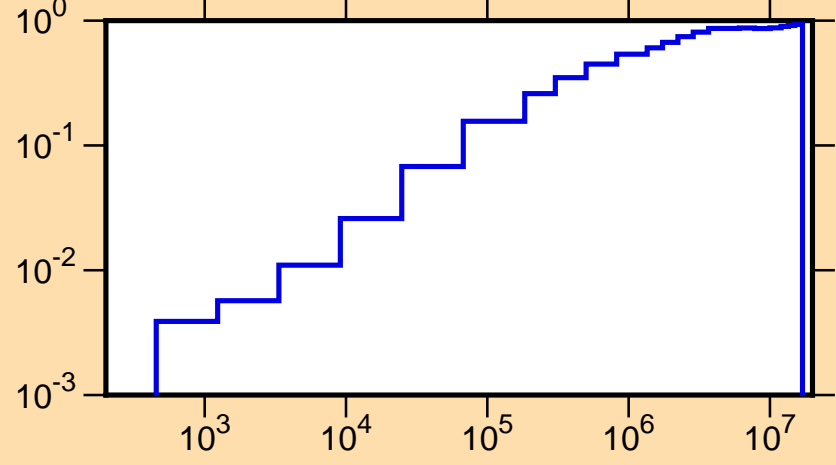
\mu vs. E for ^{230}\text{U} (mt251)
