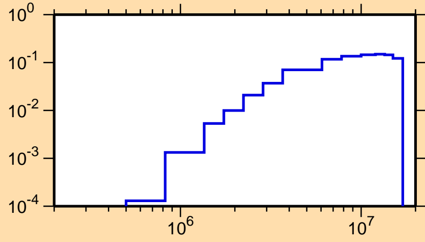
\sigma vs. E for ^{47}\text{Ti}(n,p)
