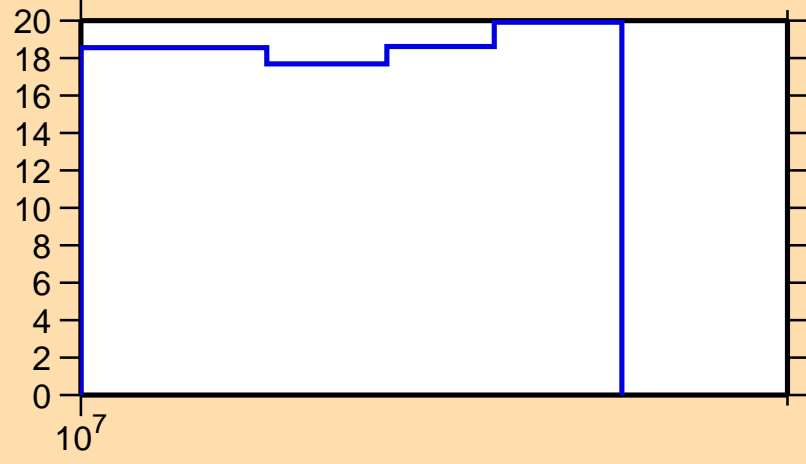
\Delta\sigma/\sigma vs. E for ^{47}\text{Ti}(n,el.)
