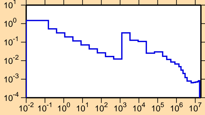
\sigma vs. E for ^{47}\text{Ti}(n,\gamma)
