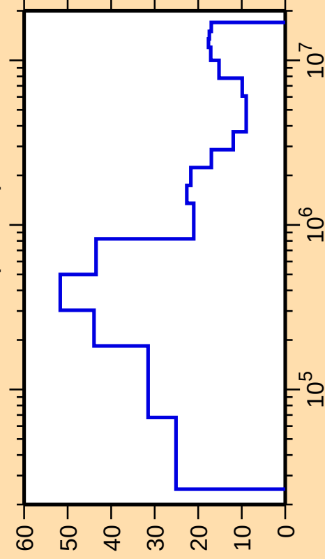
\Delta\sigma/\sigma vs. E for ^{234}\text{Th}(n,\text{inel.})
