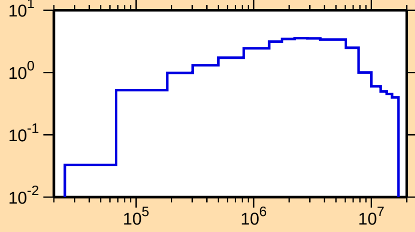
\sigma vs. E for ^{234}\text{Th}(n,\text{inel.})
