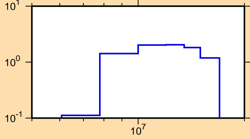
\sigma vs. E for ^{230}\text{Th}(n,2n)
