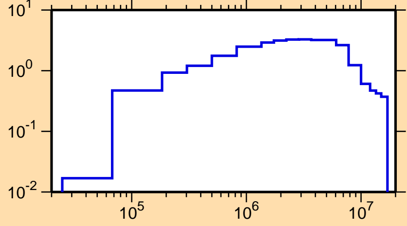
\sigma vs. E for ^{230}\text{Th}(n,\text{inel.})
