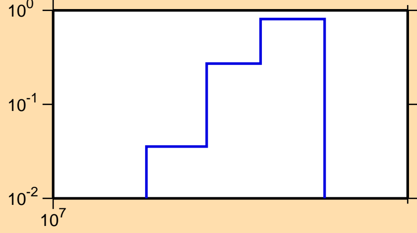
\sigma vs. E for ^{230}\text{Th}(n,3n)
