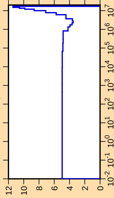
\Delta v/v vs. E for ^{229}\text{Th}(\text{total } v)
