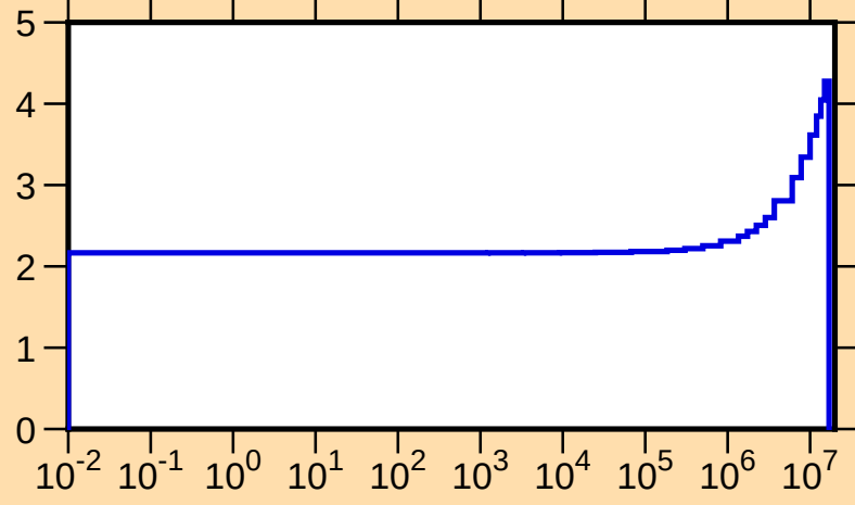
v vs. E for ^{229}\text{Th}(\text{total } v)
