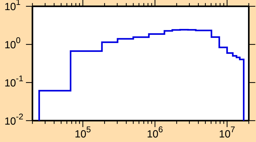
\sigma vs. E for ^{242}\text{Pu}(n,\text{inel.})
