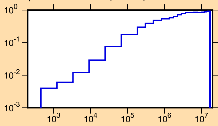
\mu vs. E for ^{237}\text{Pu}(\text{mt251})
