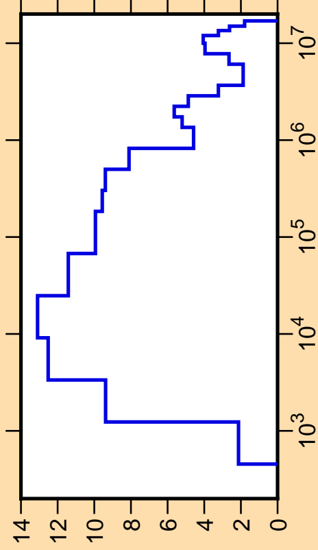
\Delta\mu/\mu vs. E for ^{237}\text{Pu}(\text{mt251})
