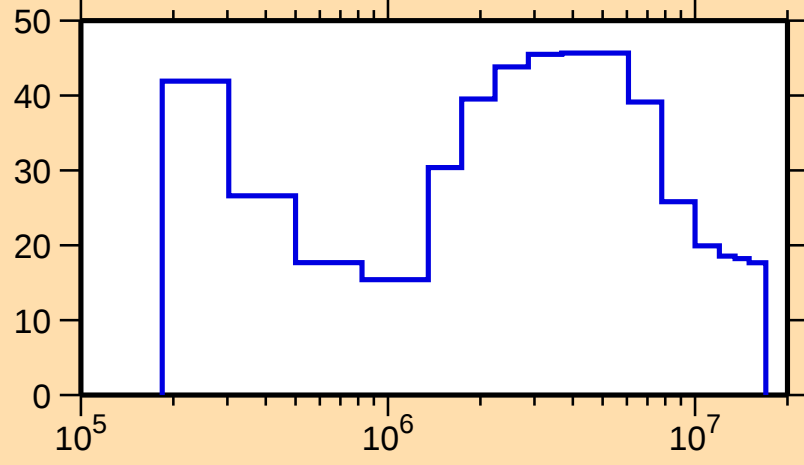
\Delta\sigma/\sigma vs. E for ^{237}\text{Pu}(n,\text{inel.})
