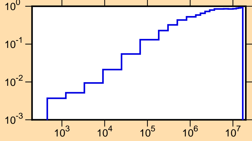
\mu vs. E for ^{232}\text{Pa}(\text{mt251})
