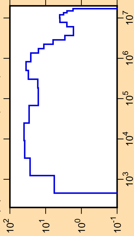
\Delta\mu/\mu vs. E for ^{232}\text{Pa}(\text{mt251})
