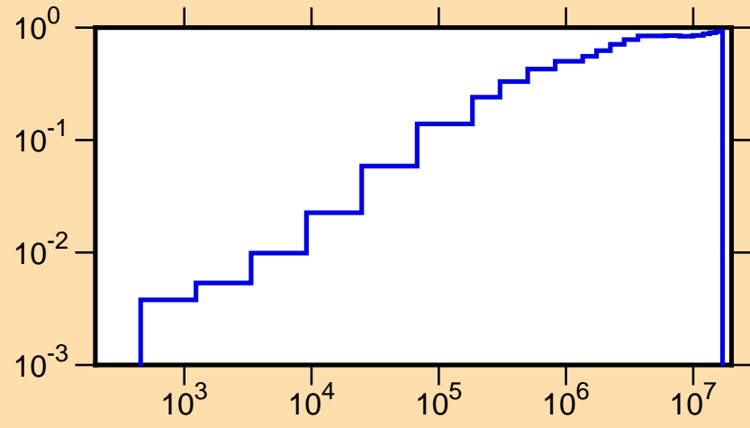
\mu vs. E for ^{229}\text{Pa}(\text{mt251})
