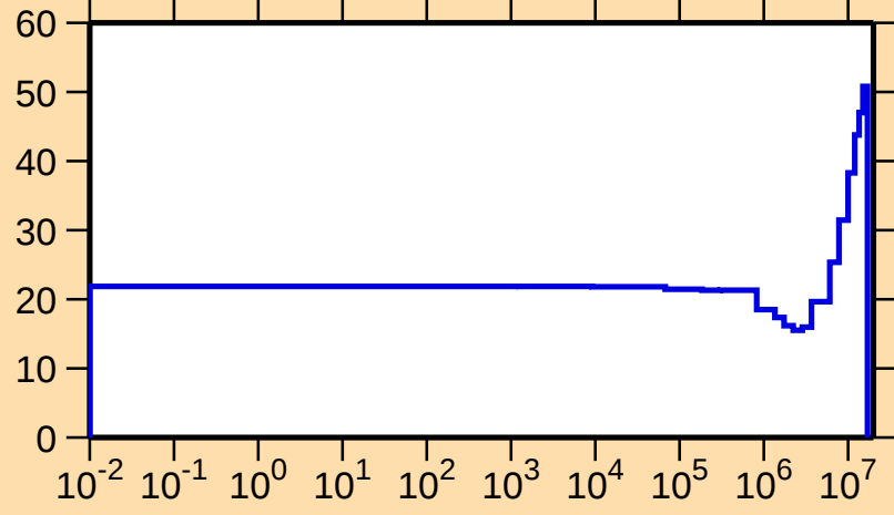
\Delta v/v vs. E for ^{238}\text{Np}(\text{total } \nu)
