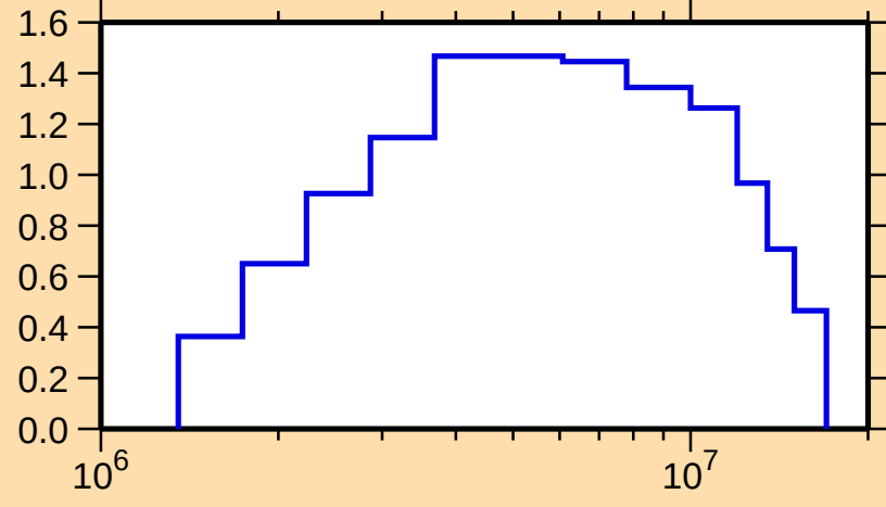
\sigma vs. E for ^{60}\text{Ni}(n,\text{inel.})
