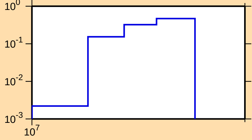
\sigma vs. E for ^{60}\text{Ni}(n,2n)
