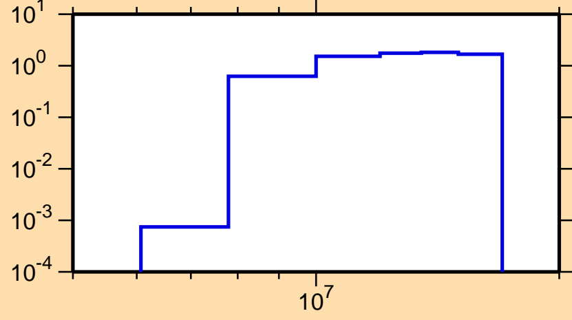
\sigma vs. E for ^{146}\text{Nd}(n,2n)
