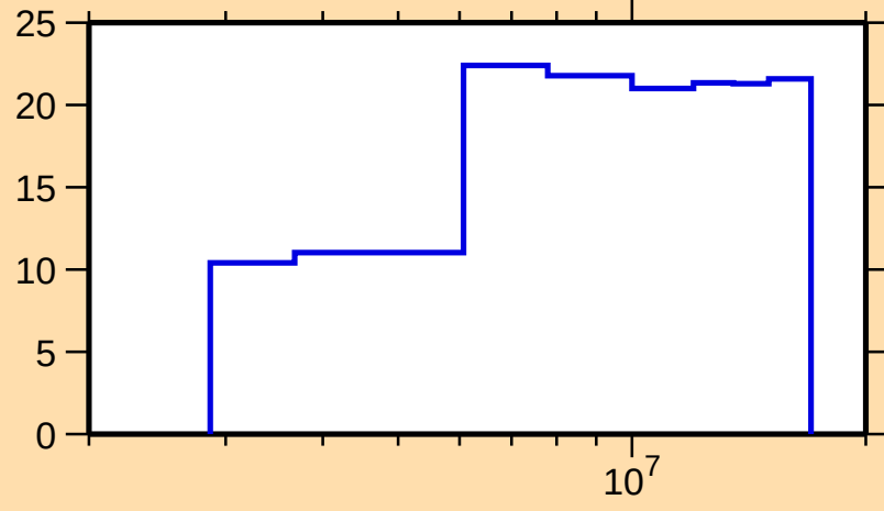
\Delta\sigma/\sigma vs. E for ^{55}\text{Mn}(\text{mt852})
