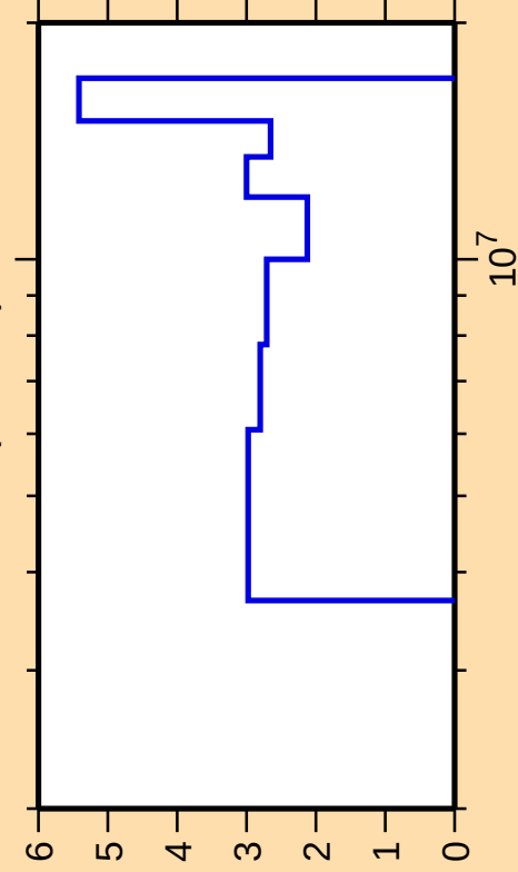
\Delta\sigma/\sigma vs. E for ^{55}\text{Mn}(\text{mt851})
