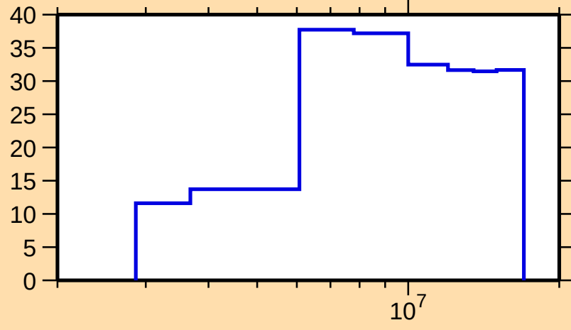
\Delta\sigma/\sigma vs. E for ^{55}\text{Mn}(\text{mt853})
