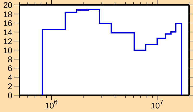
\Delta\sigma/\sigma vs. E for ^{55}\text{Mn}(\text{n,el.})
