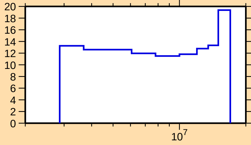
\Delta\sigma/\sigma vs. E for ^{55}\text{Mn}(\text{mt854})
