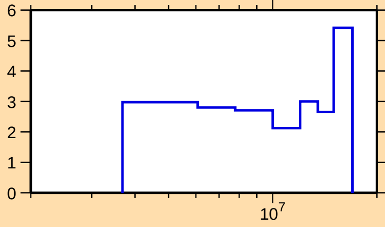
\Delta\sigma/\sigma vs. E for ^{55}\text{Mn}(\text{mt851})
