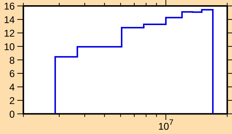
\Delta\sigma/\sigma vs. E for ^{55}\text{Mn}(\text{n},\text{n}_1)
