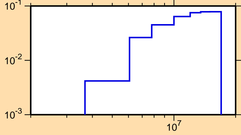
\sigma vs. E for {}^6\text{Li}(n,2n\alpha)
