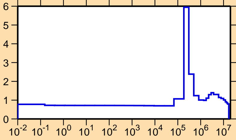
\sigma vs. E for {}^6\text{Li}(n,\text{el.})
