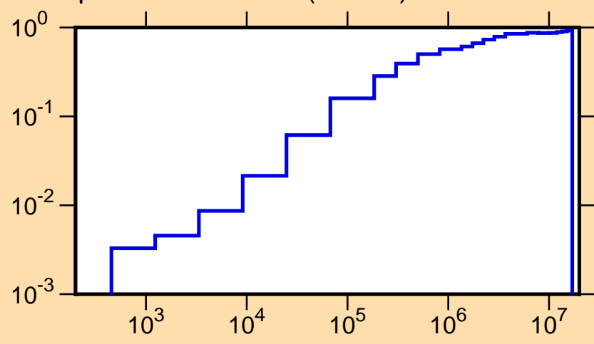
\mu vs. E for ^{249}\text{Cm}(\text{mt251})
