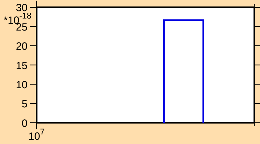
\sigma vs. E for ^{249}\text{Cm}(n,4n)
