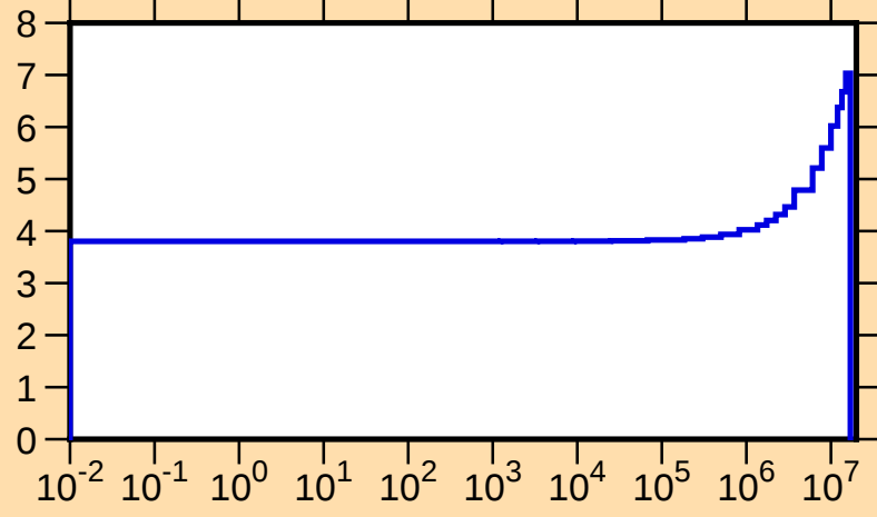
v vs. E for ^{247}\text{Cm}(\text{total } v)
