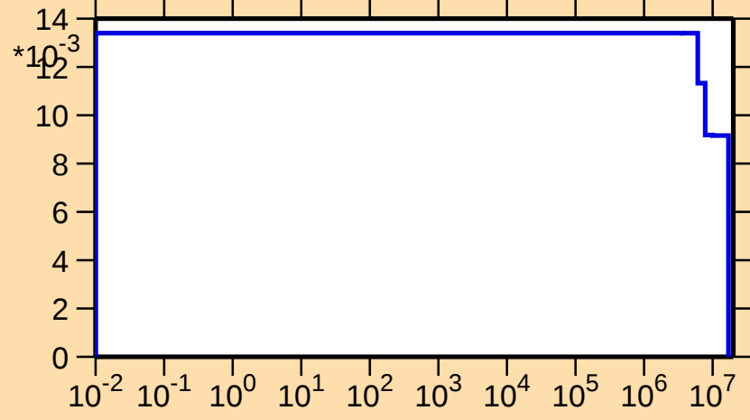
\nu vs. E for ^{247}\text{Cm}(\text{delayed } \nu)
