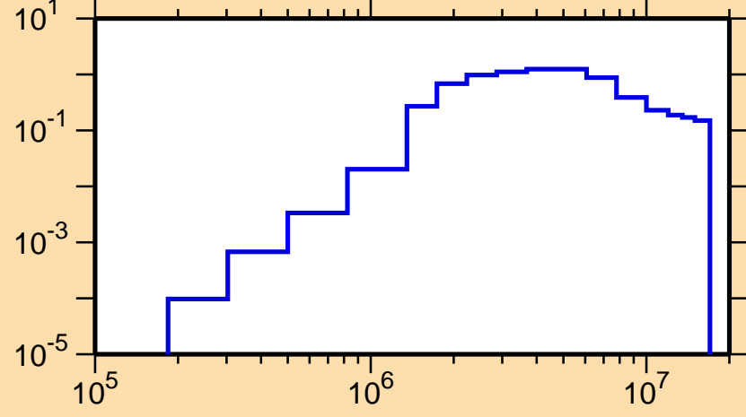
\sigma vs. E for ^{244}\text{Cm}(n,n\text{cont.})
