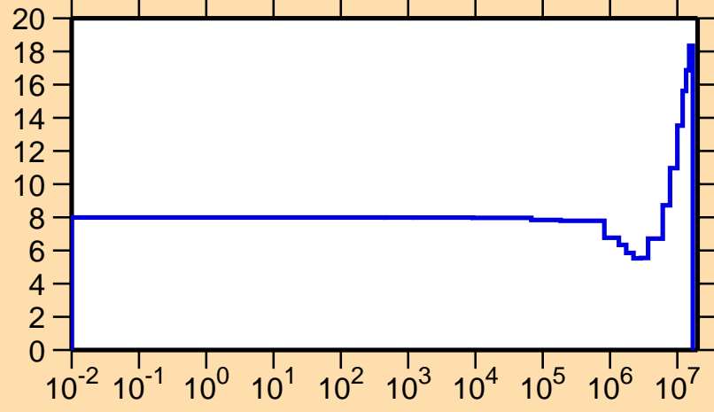
\Delta v/v vs. E for ^{244}\text{Cm} (total v)
