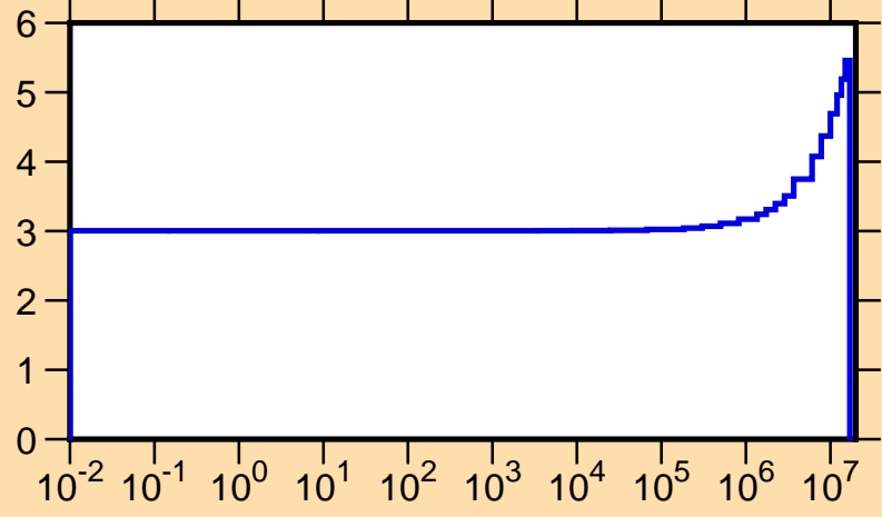
\nu vs. E for ^{244}\text{Cm}(\text{total } \nu)
