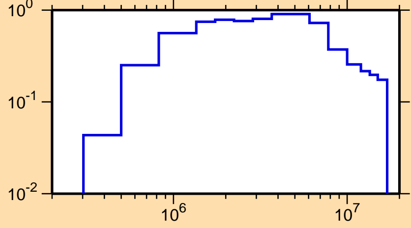
\sigma vs. E for ^{243}\text{Cm}(n,n\text{cont.})
