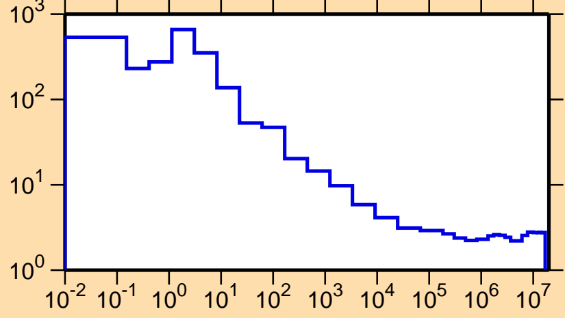
\sigma vs. E for ^{243}\text{Cm}(n,f)
