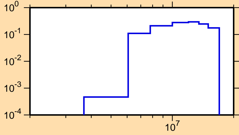
\sigma vs. E for ^{243}\text{Cm}(n,2n)
