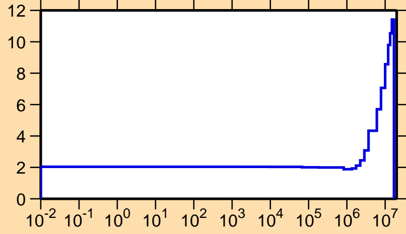
\Delta v/v vs. E for ^{243}\text{Cm}(\text{total } \nu)
