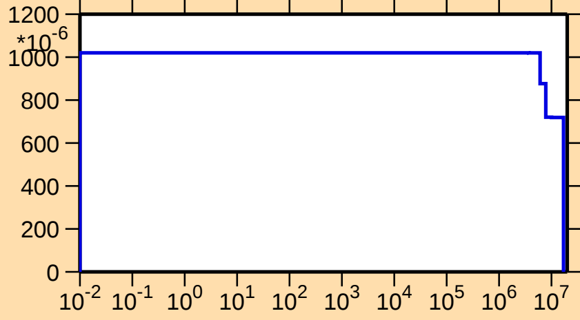
\nu vs. E for ^{240}\text{Cm}(\text{delayed } \nu)
