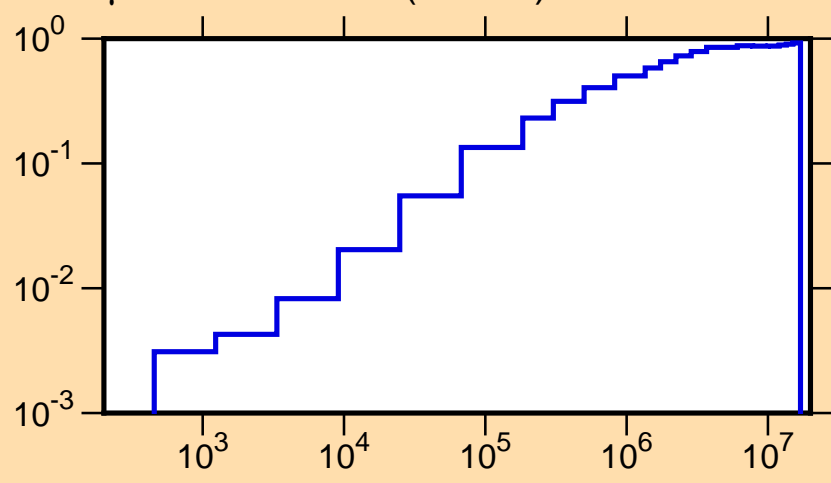
\mu vs. E for ^{254}\text{Cf}(\text{mt251})
