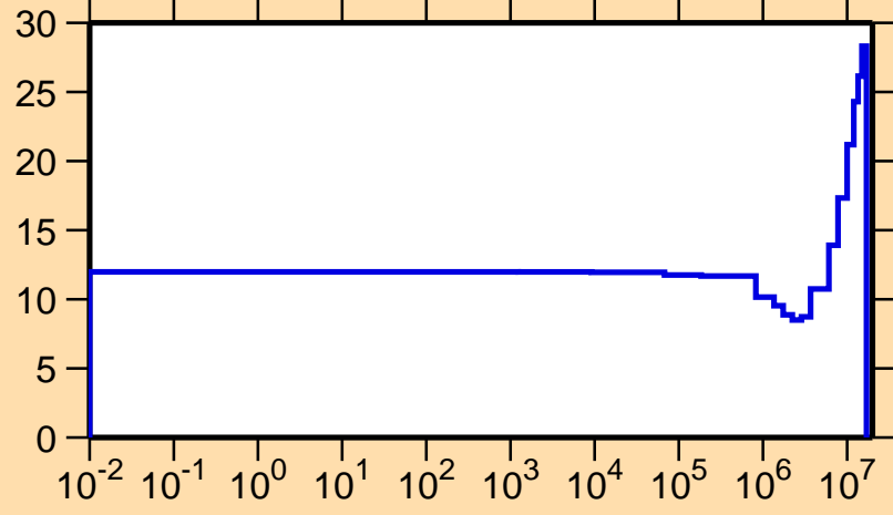
\Delta v/v vs. E for ^{251}\text{Cf} (total v)
