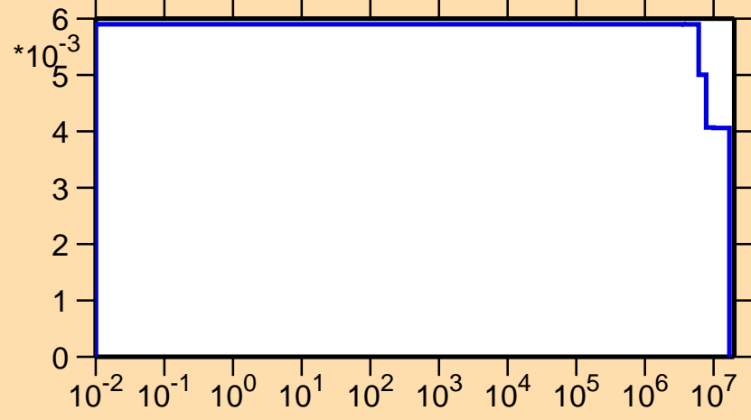
\nu vs. E for ^{251}\text{Cf}(\text{delayed } \nu)
