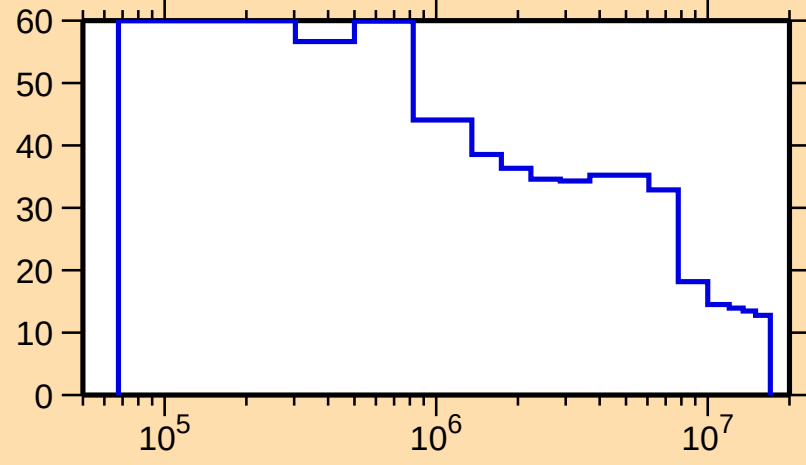
\Delta\sigma/\sigma vs. E for ^{246}\text{Bk}(n,\text{inel.})
