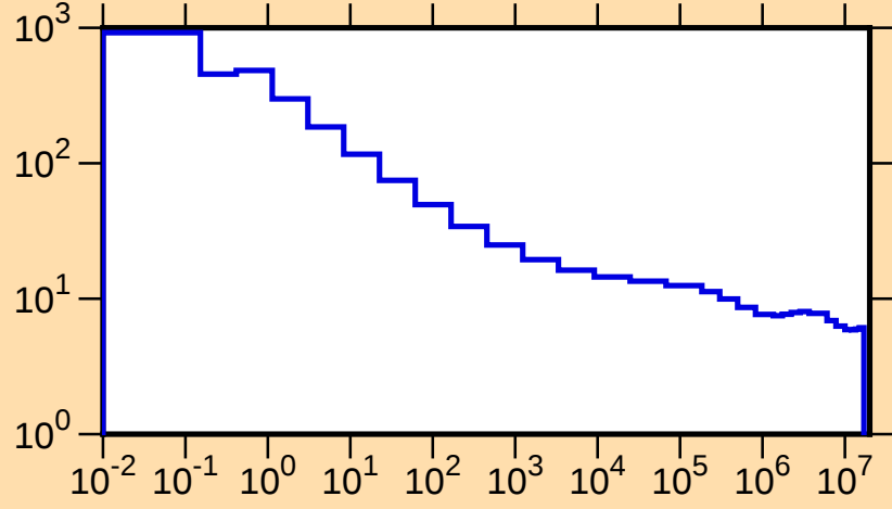
\sigma vs. E for ^{245}\text{Bk}(n,\text{tot.})
