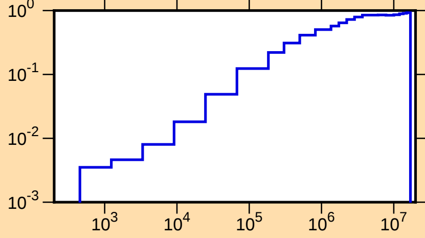
\mu vs. E for ^{227}\text{Ac}(\text{mt251})
