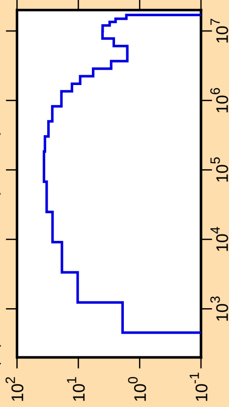
\Delta\mu/\mu vs. E for ^{227}\text{Ac}(\text{mt251})
