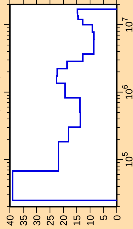
\Delta\sigma/\sigma vs. E for ^{225}\text{Ac}(n,\text{inel.})
