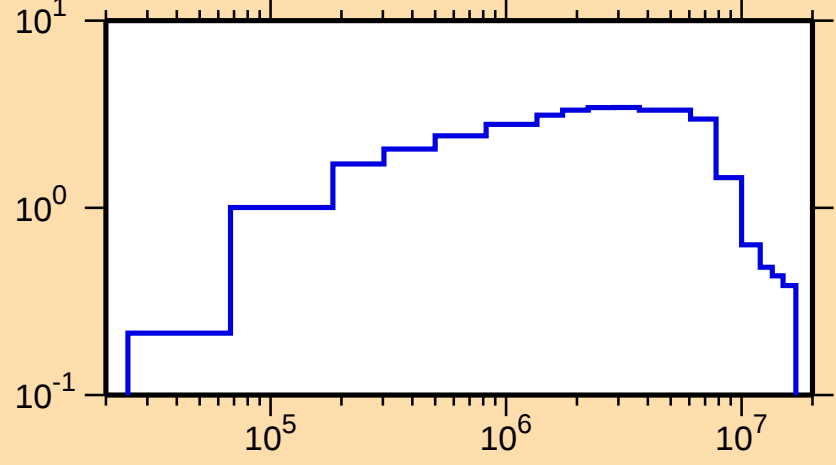
\sigma vs. E for ^{225}\text{Ac}(n,\text{inel.})
