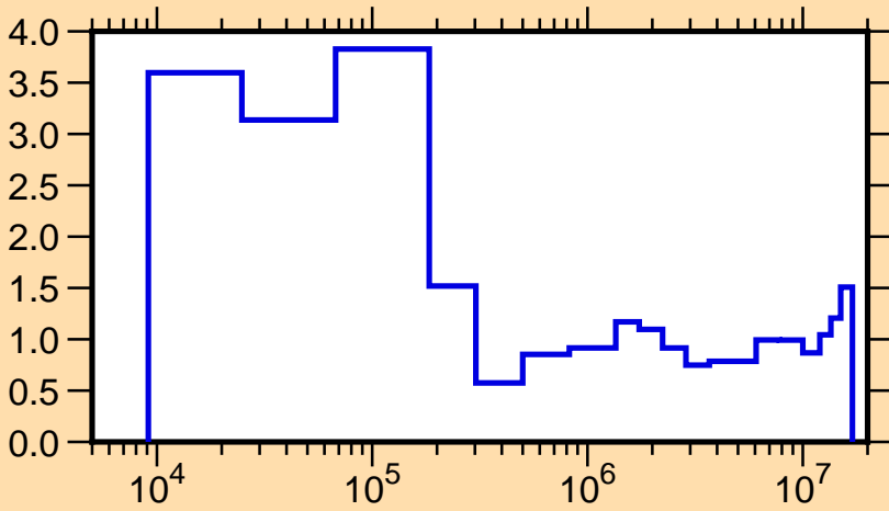
\Delta\mu/\mu vs. E for ^{238}\text{U} (mt251)
