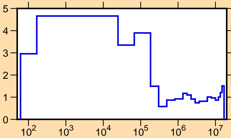
\Delta\mu/\mu vs. E for ^{238}\text{U} (mt251)
